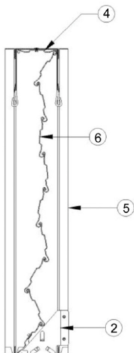
FDI - Closed Vertical Mounting
